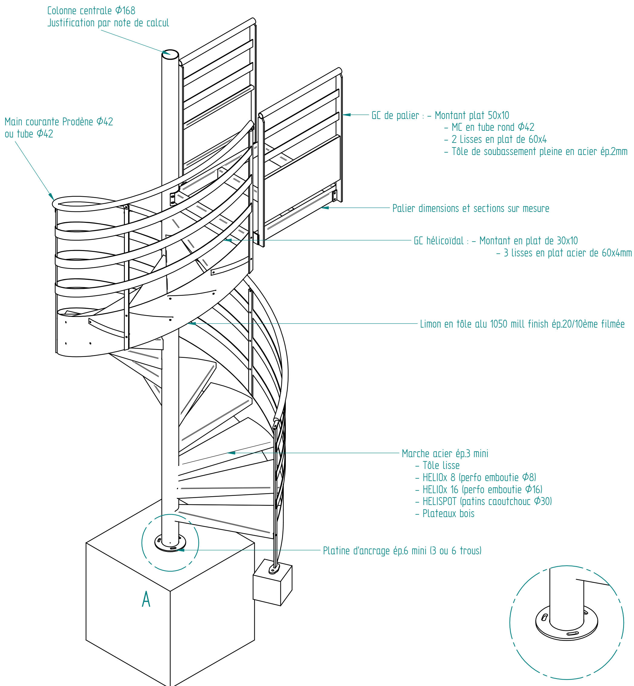
DETAIL A
